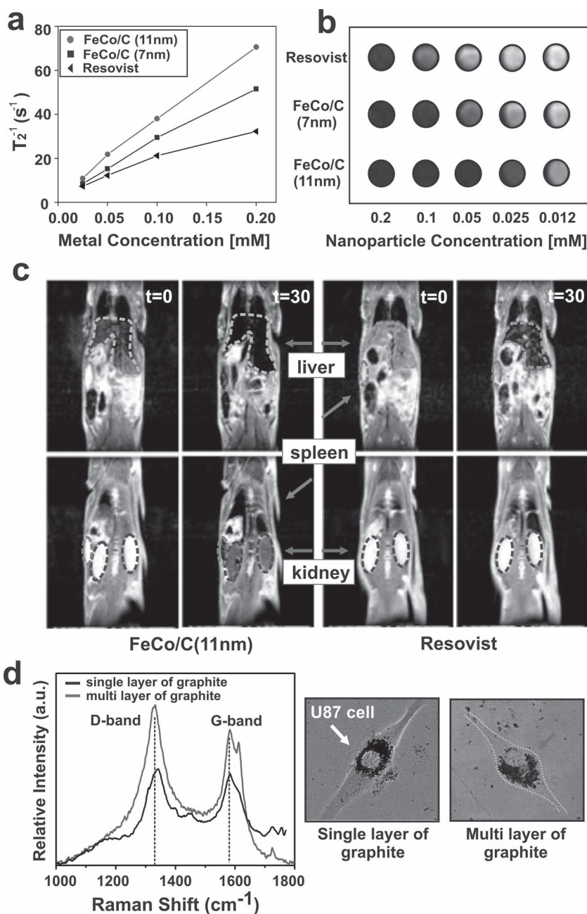
Figure 3. MR measurements and imaging of FeCo/C NPs and Resovist. a) Concentration-dependent T_2 measurements of FeCo/C NPs and Resovist solutions. b) T_2 -weighted MR images of various nanoparticle solutions. The FeCo/C NPs show higher MR image contrast (several fold) as compared to Resovist, a traditional MRI contrast agent. c) T_2 -weighted MR images of a rat before ( t = 0 min) and 30 min after ( t = 30 min) injection of FeCo/C NPs (left) and Resovist (right) into a rat's tail vein. The nanoparticles were seen to localize in the liver (green arrow), spleen (blue arrow), and kidneys (red arrow) of the animal. Also, FeCo/C NPs show a higher imaging contrast at a lower concentration (0.25 mg of Fe) as compared to Resovist (2.5 mg of Fe). d) Raman spectra of U87-EGFP cells (marked by arrows) treated with 11-nm FeCo/C NPs. The spectra shows the capability of the FeCo/C NPs to be used as imaging agents at the single-cell level (see Figure S8 in the SI for detailed Raman imaging).
