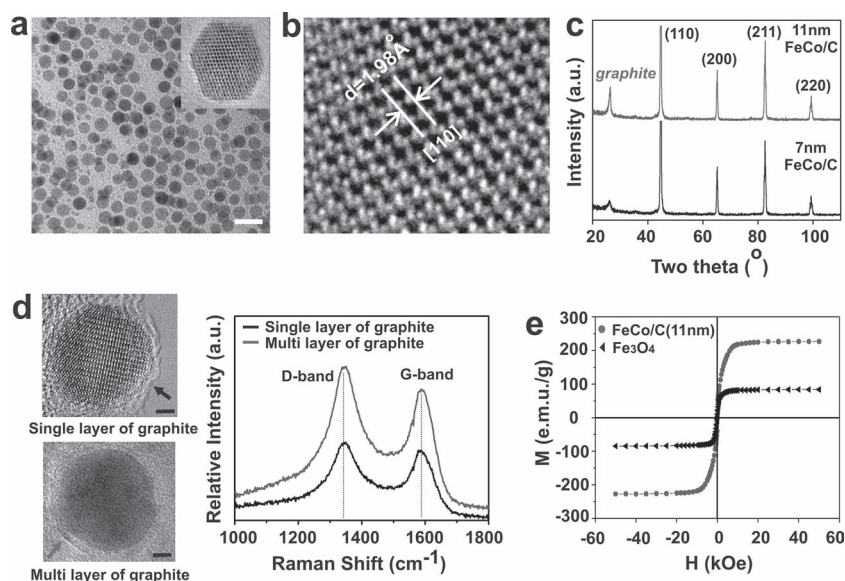
Figure 2. Structural and magnetic properties of the FeCo/C nanoparticles. a) TEM image of the 11-nm nanoparticles (scale bar = 20 nm). b) HR-TEM image of the nanoparticles showing the crystalline lattice structure of the FeCo core. c) Powder XRD for the 7- and 11-nm nanoparticles showing the presence of a bcc crystalline core and graphitic shell. d) Raman spectrum (excitation at 632.8 nm) of the 11-nm nanoparticles with single and multiple carbon shells (marked by arrows) showing the D and G bands of graphitic carbon (scale bar = 2 nm). e) Room-temperature magnetization versus applied magnetic field for 11-nm FeCo/C NPs (red symbols) and \text{Fe}_3\text{O}_4 (black symbols). Note that no hysteresis loop exists owing to the superparamagnetism of the nanoparticles.
